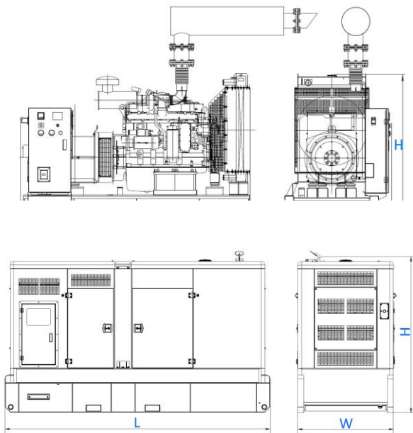
Sound-proof ( KP-DS380-SR )
